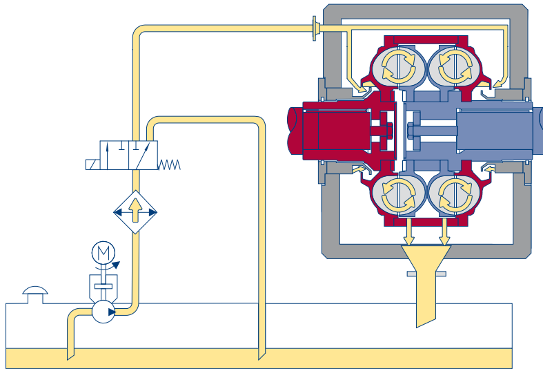
Fig. 34: Fill-controlled fluid coupling, type TP, externally supported, double circuit coupling
